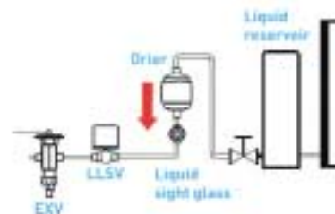
Liquid line - position of accessories
